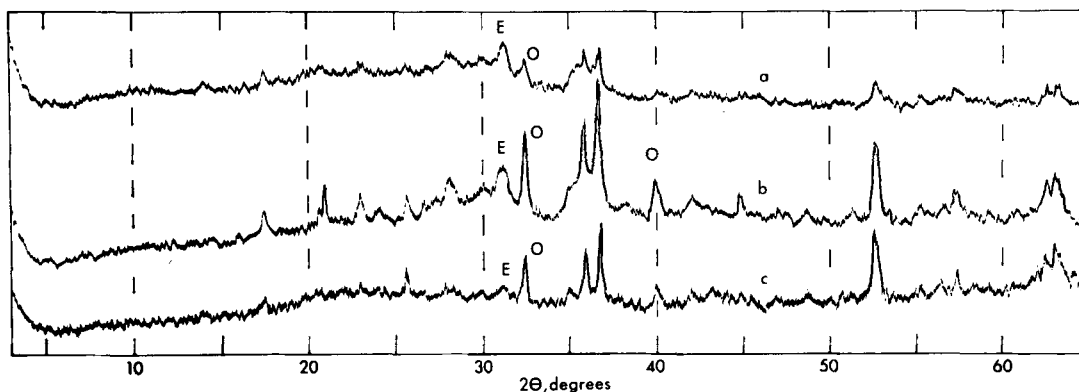
Fig. 5. Diffractometer patterns of samples (a) RO3A, (b) RO24, (c) GUS, after heat treatment at 1000°C. CuK \alpha radiation. Q = quartz, E = enstatite, O = olivine.
