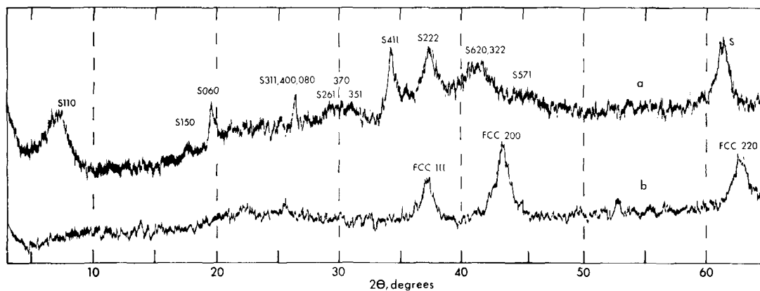
Fig. 2. Diffractometer patterns for sample Serbia 2, 27 wt % NiO estimated, after heating at (a) 800°C, (b) 1000°C; CuK \alpha radiation. S = sepiolite, FCC = face-centered cubic (see text).
