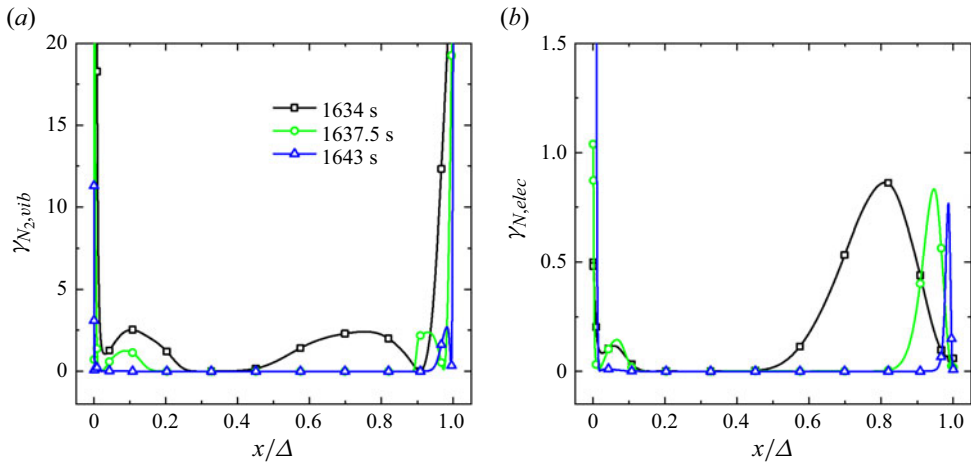
Figure 11. The spatial evolution of \gamma_{N_2,vib} (a) and \gamma_{N_2,elec} (b) along the stagnation line.
