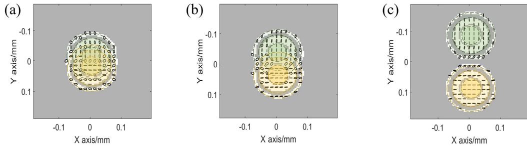
Figure 3. Polarization distribution within the focal point at various separation angles.
