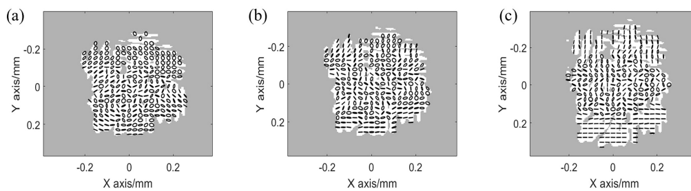
Figure 4: Polarization distribution of speckle when CPP is combined with PS at different separation angles.
