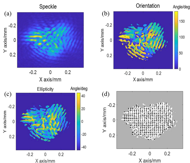
Figure 7. Speckle after CPP and PS (a) intensity distribution; (b) orientations; (c) ellipticities; (d) distribution of polarization states.
