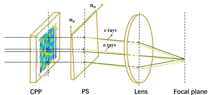
Figure 1. Schematic showing the use of a BW to achieve PS in OMEGA.
