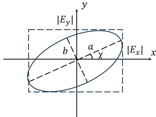
Figure 2. Polarization ellipse.
