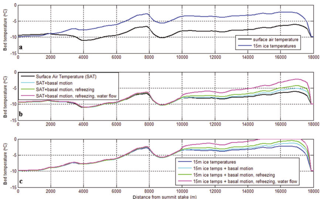
Fig. 4. Equilibrium ice–bed interface temperatures: (a) for the two different surface BCs; (b) for the mean SAT and for various additional basal heat sources below the ELA; and (c) for 15 m depth ice temperatures and for various additional basal heat sources below the ELA.
