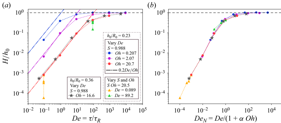
Figure 11. Numerical values of H/h_0 against (a) the Deborah number De = \tau/\tau_R based on the inertio-capillary time scale \tau_R , and (b) the general Deborah number De_N = \tau/\tau_N based on the general time scale \tau_N = \tau_R(1 + \alpha Oh) with \alpha = 4.3 , for various parameters (the same in (a) and (b)). Dots ( \bullet ) correspond to h_0/R_0 = 0.23 and S = 0.988 , with Oh = 0.207 (blue), Oh = 2.07 (purple) and Oh = 20.7 (red), and De ranging between 8.92 \times 10^{-2} and 8.92 \times 10^3 (last De excluded for the largest Oh ). Triangles ( \blacktriangle ) correspond to h_0/R_0 = 0.23 with De = 8.92 \times 10^{-2} (yellow) and De = 8.92 \times 10^1 (green), varying both S (between 0.1 and 0.988) and Oh while keeping S Oh constant and equal to 9.88. Stars ( \star ) correspond to h_0/R_0 = 0.362 with Oh = 16.6 and S = 0.988 , and De ranging between 4.59 \times 10^{-2} and 8.92 \times 10^3 .
