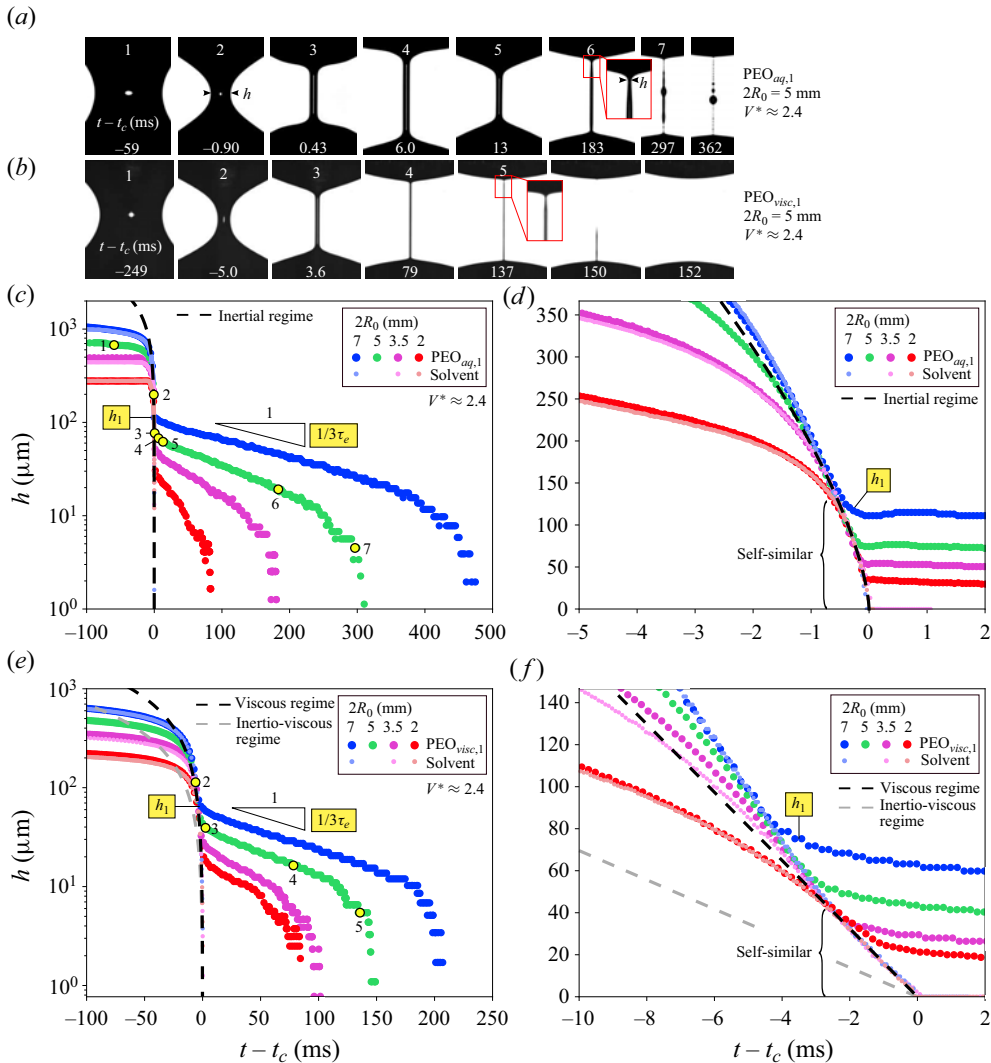
Figure 3. (a,b) Image sequences of the bridge/filament for the (a) PEO_{aq,1} and (b) PEO_{visc,1} solutions tested with plate diameter 2R_0 = 5 mm and sample volume V^* \approx 2.4 . (c–f) Time evolution of the minimum bridge/filament radius h in (c,e) semi-log and (d,f) lin–lin, for plate diameters 2R_0 between 2 and 7 mm, and fixed V^* \approx 2.4 , for the (c,d) PEO_{aq,1} and (e,f) PEO_{visc,1} solutions, and for their respective solvents (smaller data points), compared with (3.1) and (3.2), where t_c is the solvent breakup time. Times with labels 1–7 and 2–5 in (c,e), respectively, for 2R_0 = 5 mm, correspond to the snapshots in (a,b).
