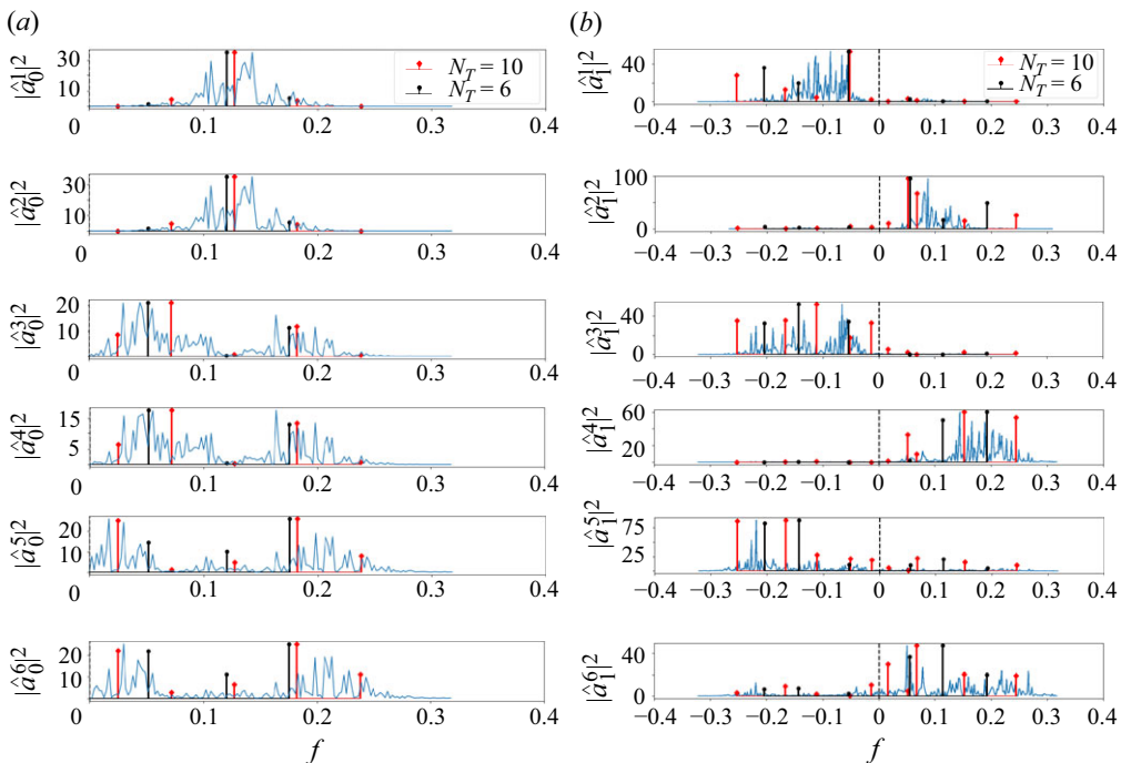
Figure 27. Predicted frequencies of the dominant POD amplitudes with the linear autonomous model (LM) for two different truncations N_T = 6 (black lines) and N_T = 10 (red lines): |\hat{a}_0^n|^2 for n \in \{1, \dots, 6\} and |\hat{a}_1^n|^2 for n \in \{1, \dots, 6\} .
