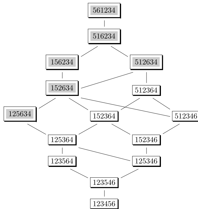
FIGURE 4.1. The EO strata for (n, m) = (4, 2) .
