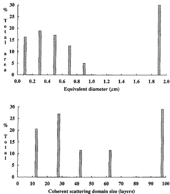
Figure 2. Comparison between equivalent diameter (Lanson and Champion, 1991) and CSDS distributions. The first distribution was obtained by TEM measurement of particle size. For each equivalent diameter class, the surface corresponding to all the particles of this class was calculated and divided by the total surface (sum of the surface for all the observed particles). The CSDS distribution was obtained fitting the proportions of five theoretical muscovite patterns on the experimental X-ray pattern (least squares method).
