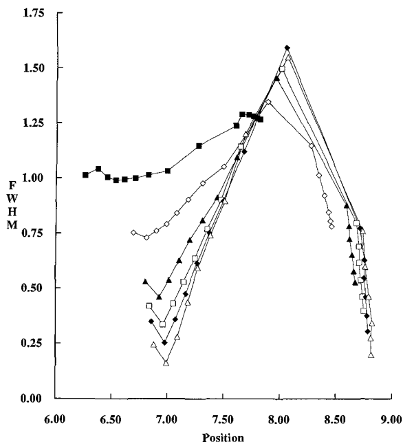
Figure 5. Identification diagrams for ordered ( R = 1 ) mixed-layer illite/smectite. Position and width (FWHM) are given in ^\circ 2\theta CuK \alpha . Illite/smectite (hydrated with two interfoliar water sheets), mixed-layer. Maximum ordering. The patterns represent CSDS distributions (solid squares: 2 \leq N \leq 5 ; open diamonds: 6 \leq N \leq 9 ; solid triangles: 11 \leq N \leq 14 ; open squares: 16 \leq N \leq 19 ; solid diamonds: 22 \leq N \leq 25 ; open triangles: 36 \leq N \leq 39 ). The compositions vary from 45–100% Illite (5% Ill steps from 45–90% Ill, and 2% Ill increments from 90–100% Ill).
