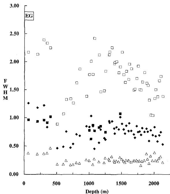
Figure 11. Evolution of full width at half maximum ( ^{\circ}2\theta \text{CuK}\alpha ) vs depth (meters) for Well C. The widths are obtained from decomposition of EG X-ray patterns. Patterns as Figure 10.
