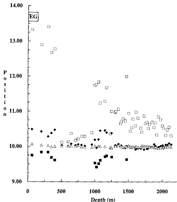
Figure 10. Evolution of position ( \text{\AA} ) vs depth (meters) for Well C. The positions are obtained from decomposition of EG X-ray patterns. The patterns indicate the phases associated with the different elementary peaks: empty triangles: detrital mica; solid diamonds: illite; empty and solid squares: mixed-layer illite/smectite (ordered).
