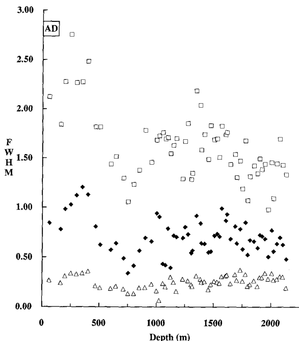
Figure 9. Evolution of full width at half maximum ( ^{\circ}2\theta CuK \alpha ) vs depth (meters) for Well C. The widths are obtained from decomposition of AD X-ray patterns. Patterns as Figure 8.
