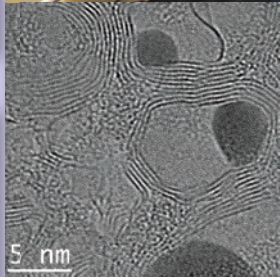
Pd nanocrystals
