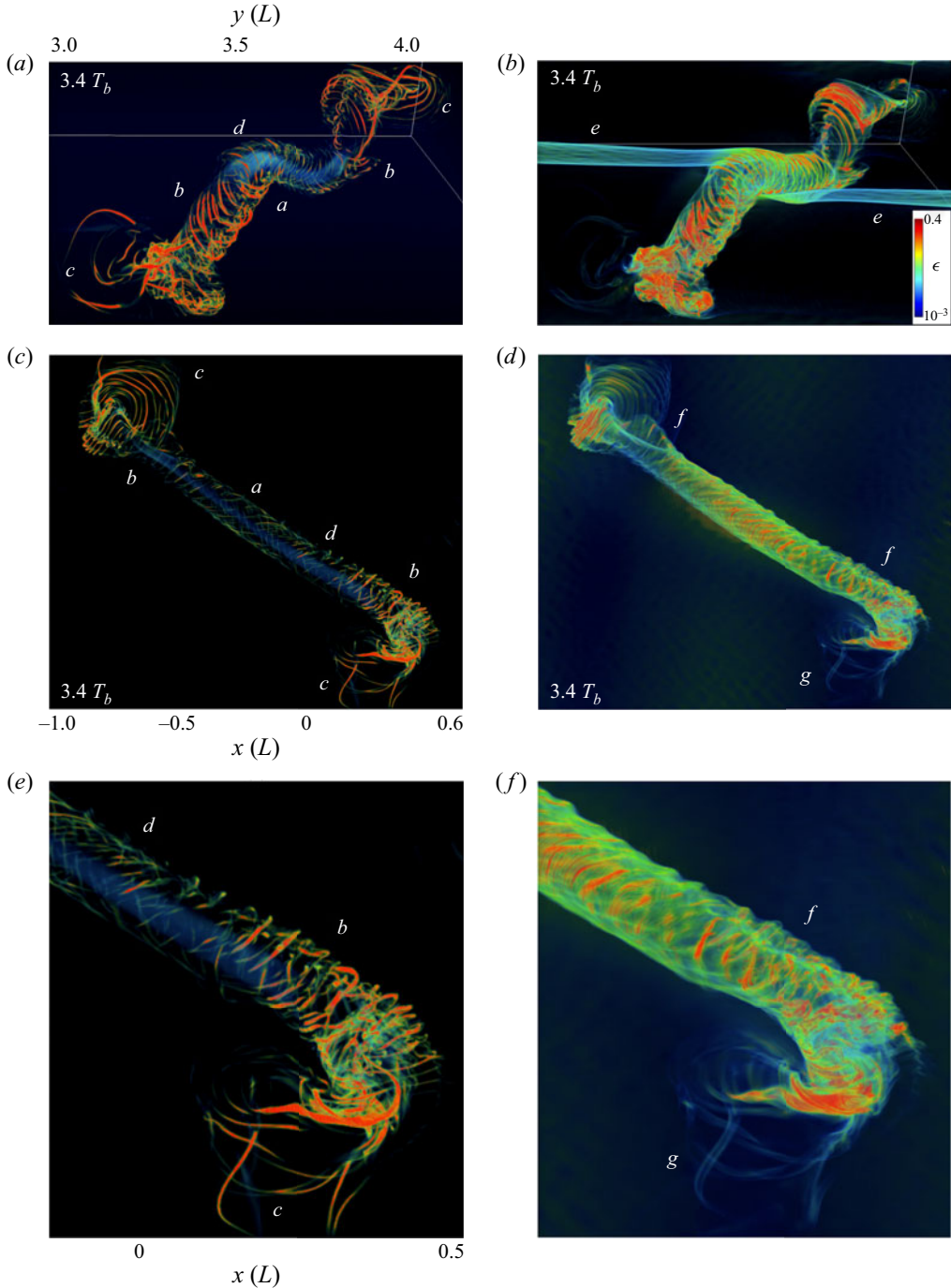
Figure 9. As in figure 8 at 3.4T_b showing the relations of \lambda_2 and \epsilon for the vortex tube in region 1 in figure 2 and the fine structure driving the turbulence transition and the \epsilon features for this event. The lower expanded images (see x/L axes at centre and bottom left) reveal spacings between initial small-scale secondary KHI in the sheath to be as small as \sim 0.01L and to have even finer vortex cores in \lambda_2 at apparently smaller radii. See text for additional details. The \epsilon colour scale is as in figure 8. Sites labelled a – g are cited in the text.
