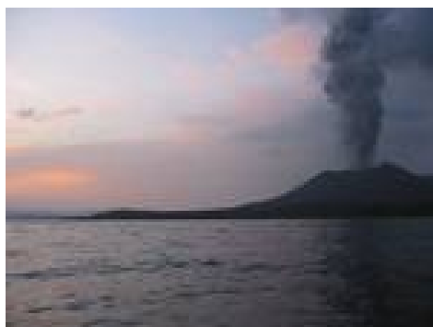
Rabaul volcano
